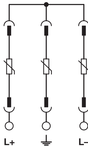
Circuit diagram
