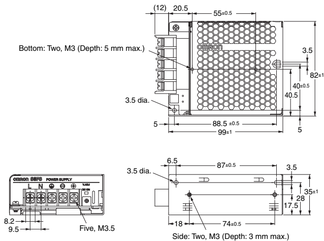
Panel mounting hole dimensions
