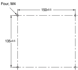
Panel mounting hole dimensions
