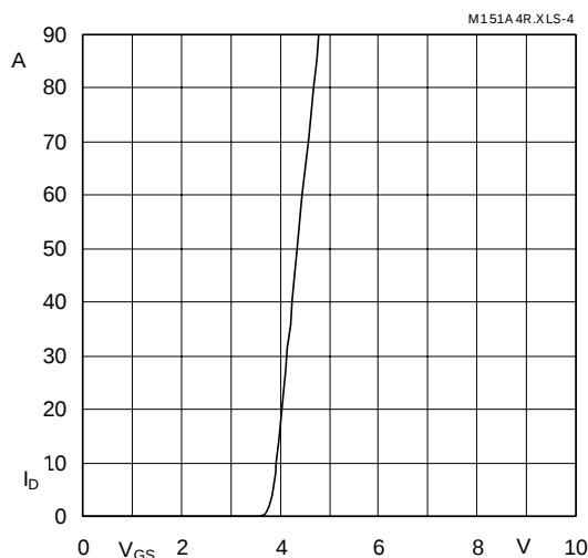
Fig. 4 Transfer characteristic
