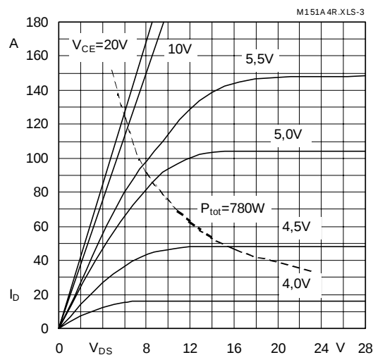
Fig. 3 Output characteristic
