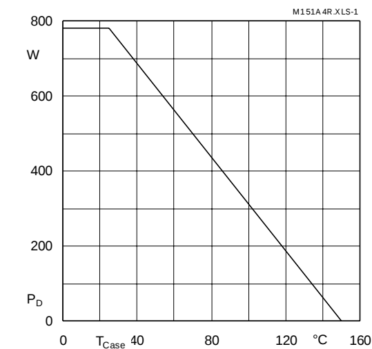
Fig. 1 Rated power dissipation vs. temperature
